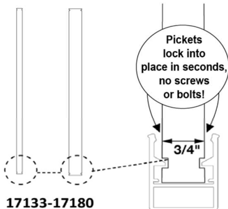
17133-17180 Pickets
